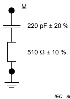
Figure 6 – Artificial hand, RC element (see 7.3.5)
