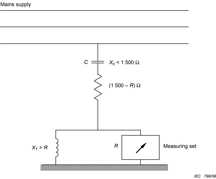
Figure 4 – Circuit for disturbance voltage measurements on mains supply (see 7.3.3)
